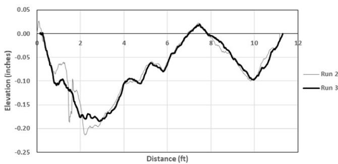
Figure 9. Graph. Two runs with the highest cross-correlation for AHSV1 at test section NB-1 (run 2 and run 3, cross-correlation = 95 percent).
