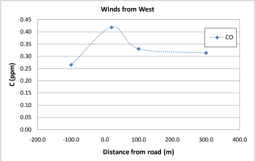
Figure 9. Average CO Concentrations -- winds from west.
