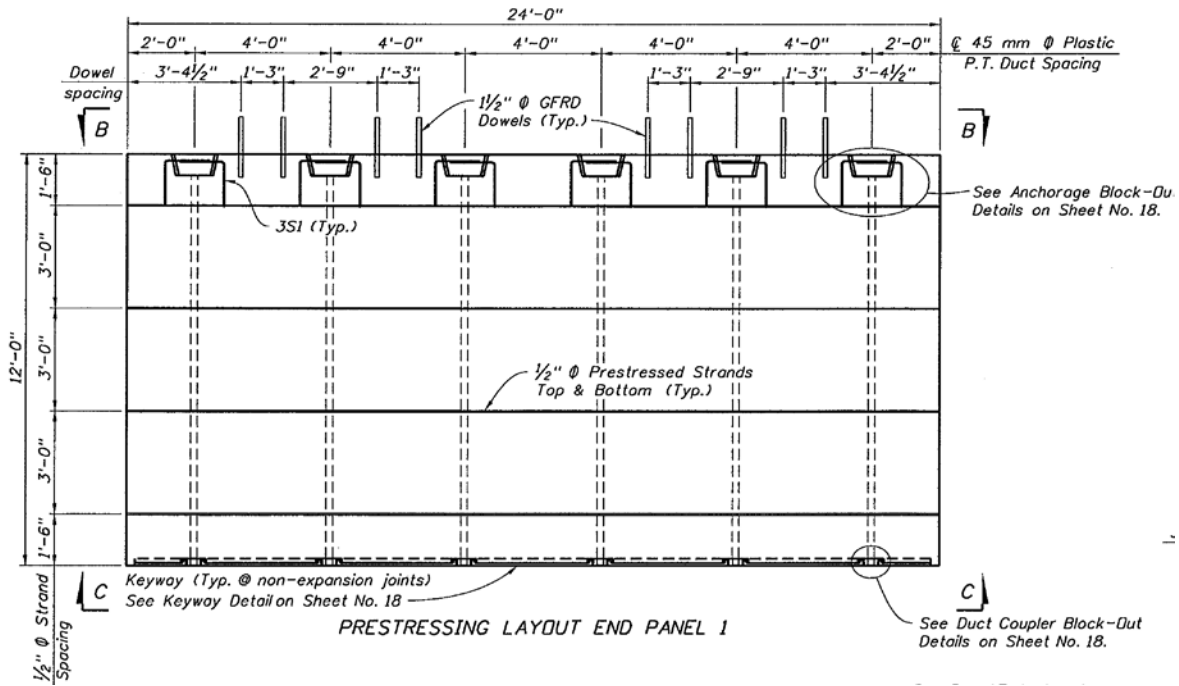
Figure 5. Diagram. Panel prestressing layout.
