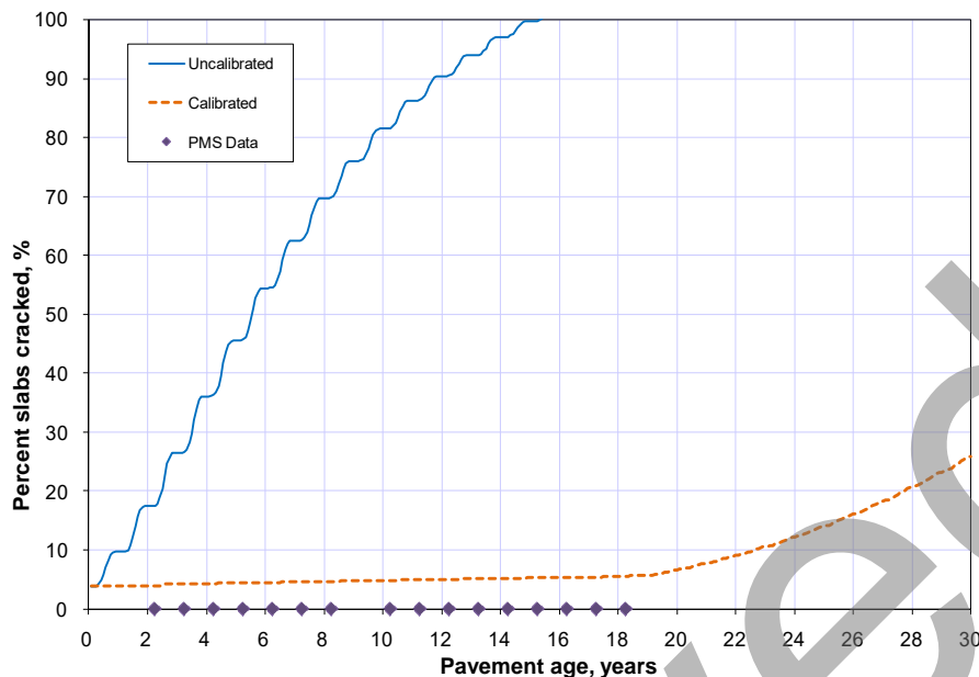
Figure 35. Locally calibrated PCC transverse cracking model – section I-900AC.
