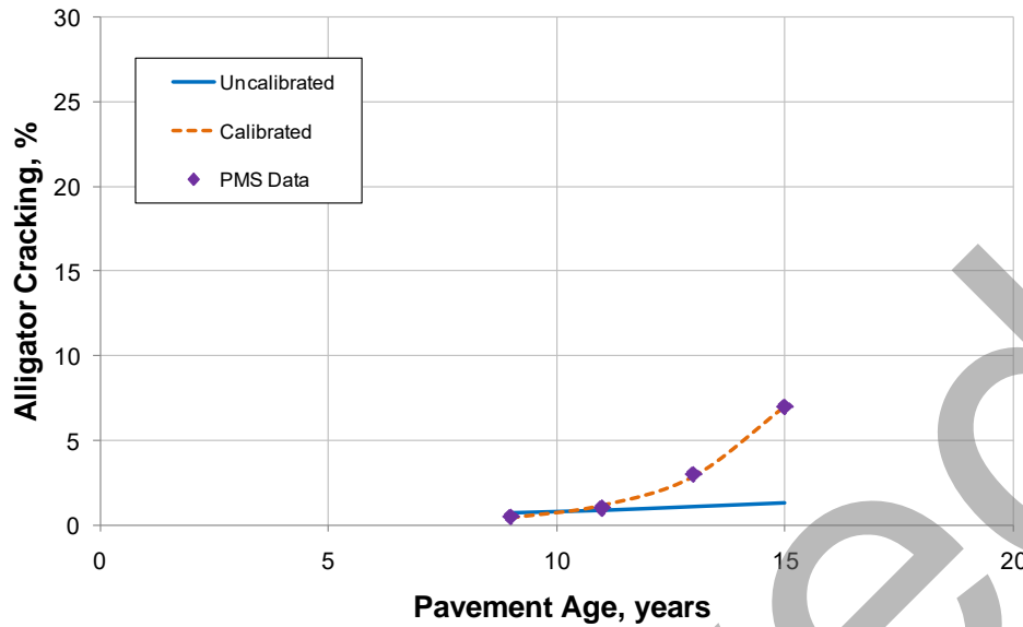
Figure 23. Locally calibrated alligator cracking model – section U508CA.
