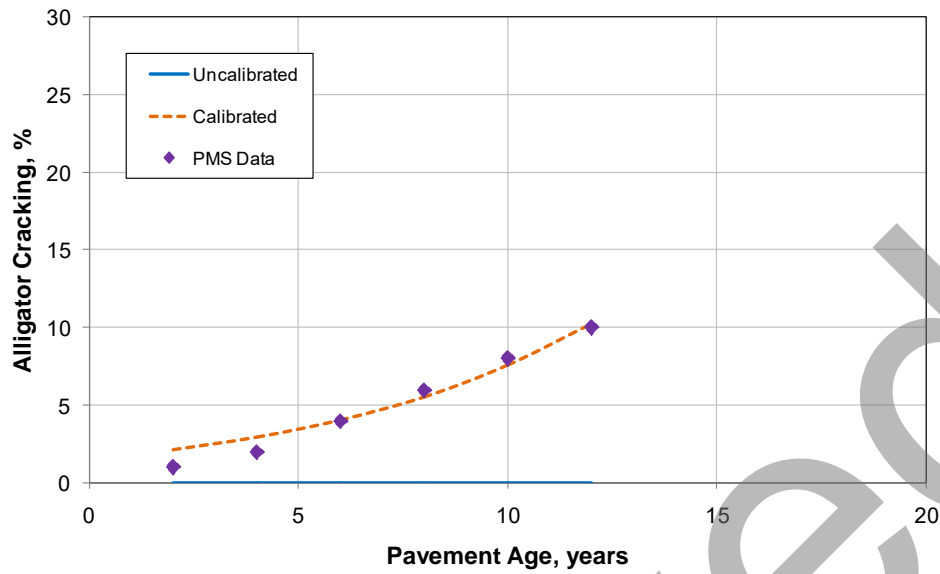
Figure 21. Locally calibrated alligator cracking model – section R2211BA.
