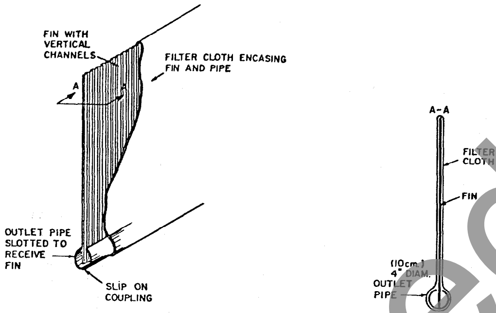
Figure 74. Typical Components of Prefabricated Fin Drains (101)
