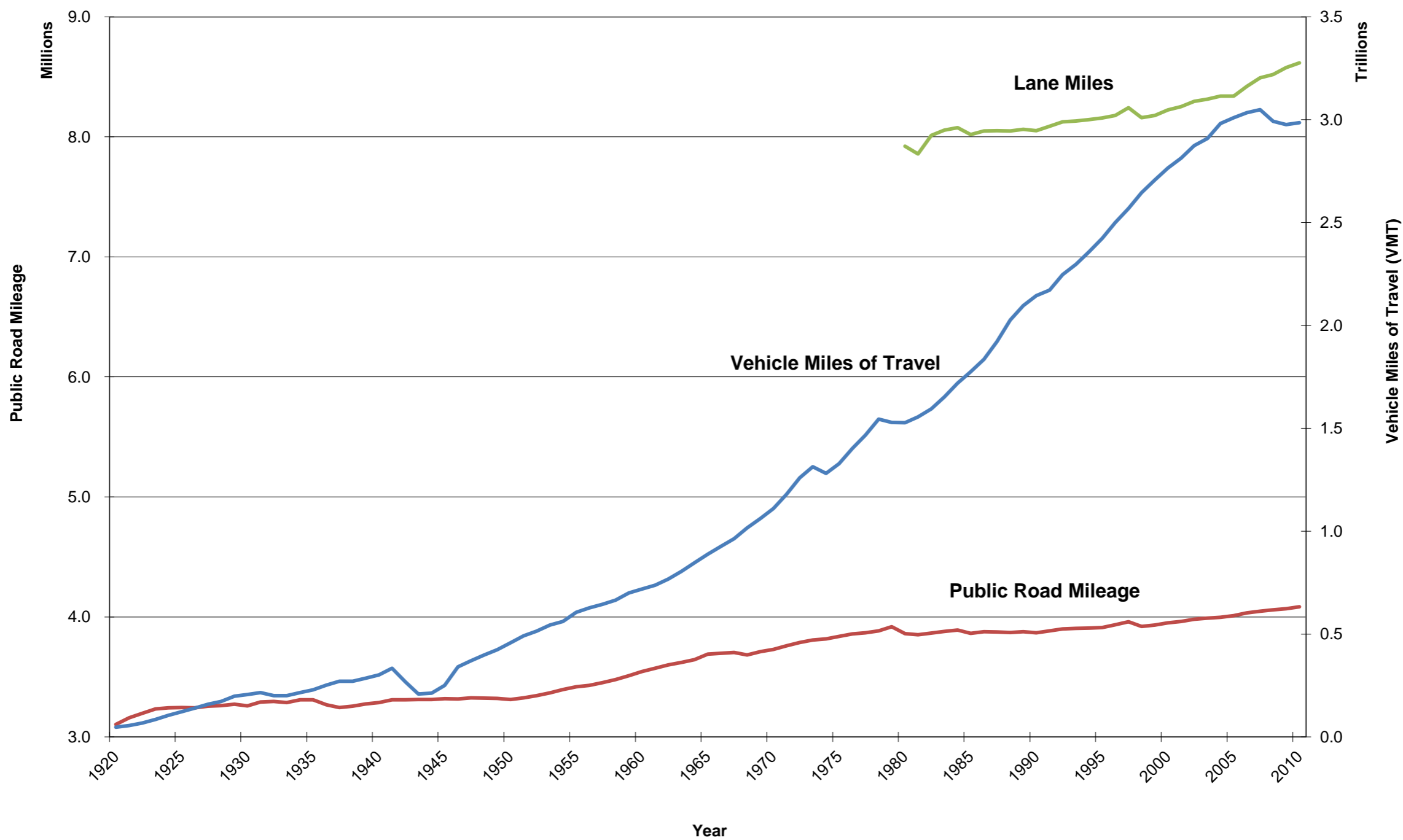
Public Road Mileage - VMT - Lane Miles 1920 - 2010
