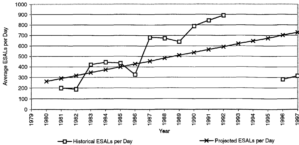
Figure 61. Comparison of projected and historical ESALs for Site 37-3807.
