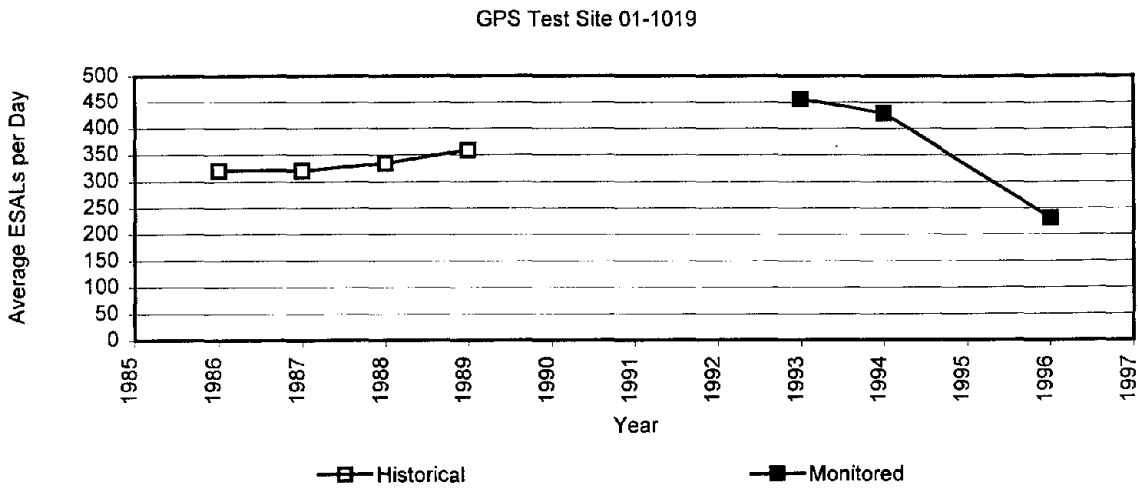
Figure 1. Comparison of trends for average historical and monitoring ESALs per day.
