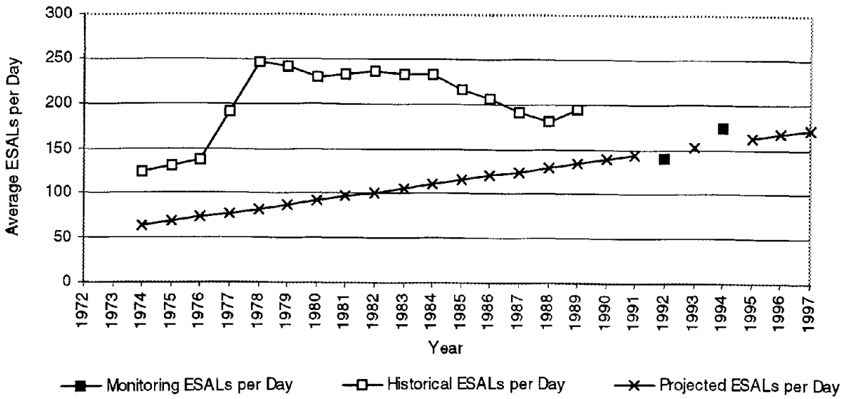
Figure 34. Comparison of ESAL volumes for Site 27-0501.
