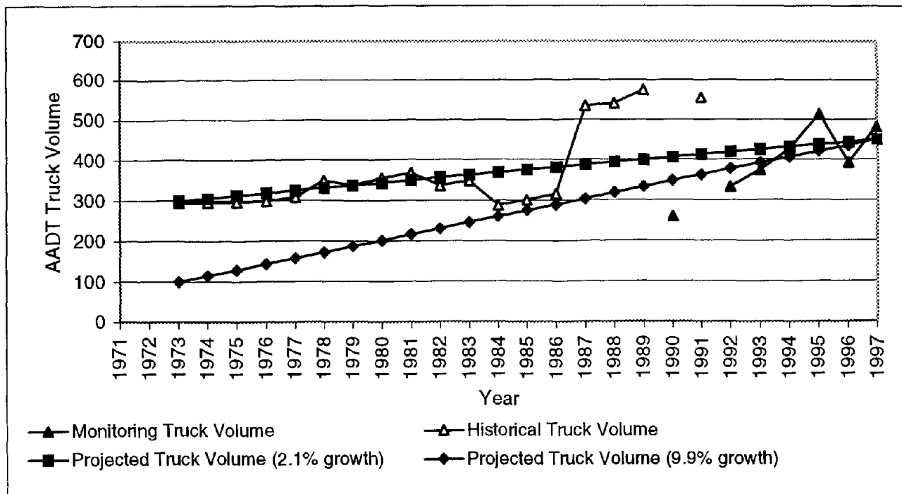
Figure 50. Projected total truck volumes for Site 29-5483.
