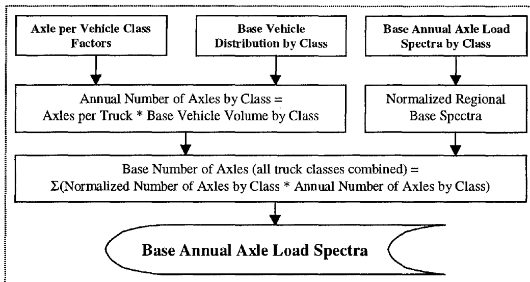
Figure 91. Flowchart for computation of the base annual axle load spectra.
