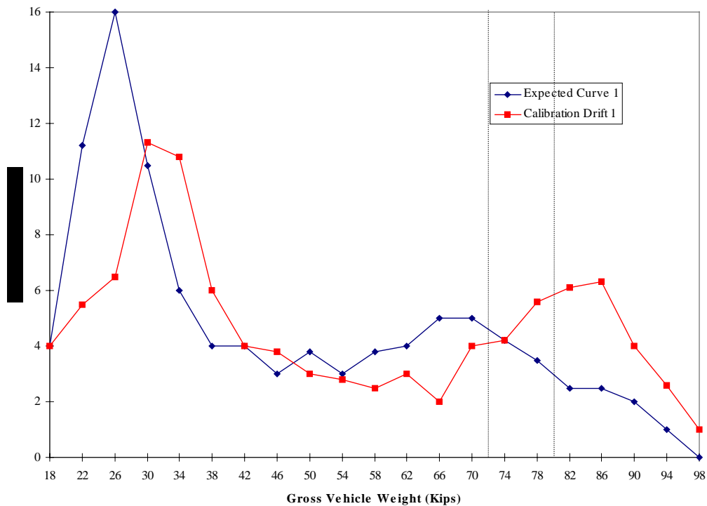
Figure 1. Calibration drift using GVW for five-axle tractor semi-trailer trucks.
