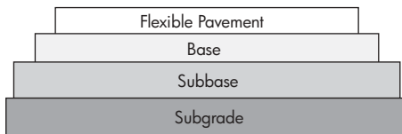
Figure 13. Schematic of a flexible pavement structure
