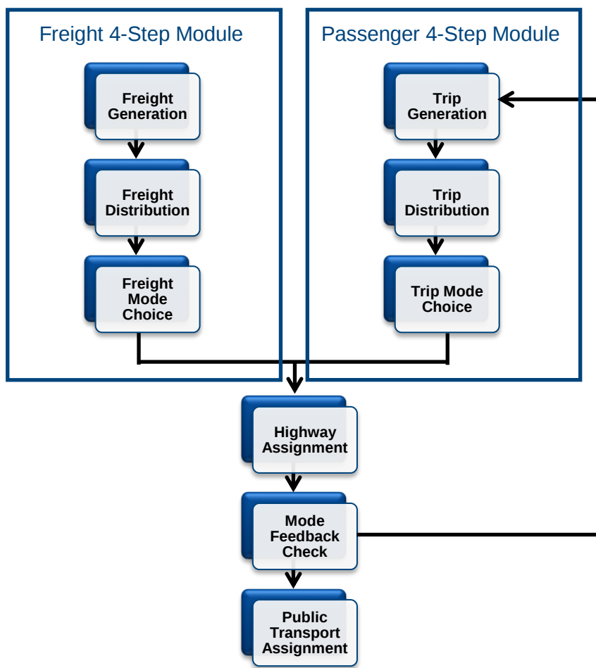
Figure: Model Flows & Structures (Source: GDOT Statewide Travel Demand Model Presentation, 2012)
