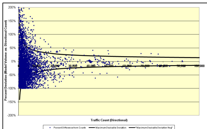
Figure 4: 2006 Link Volume Maximum Desired Deviation Scatter Plot
