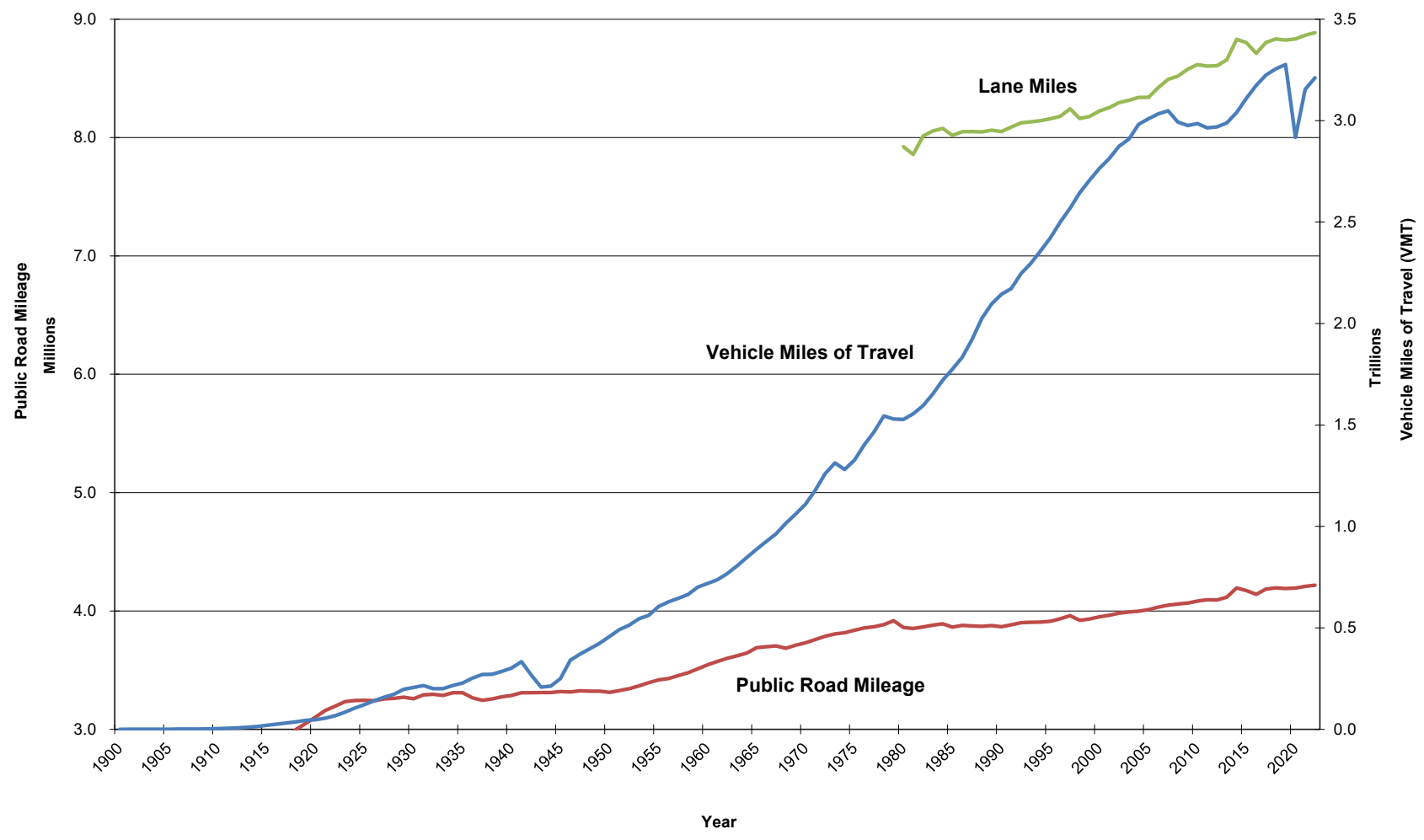
Public Road Mileage - VMT - Lane Miles 1900 - 2022
