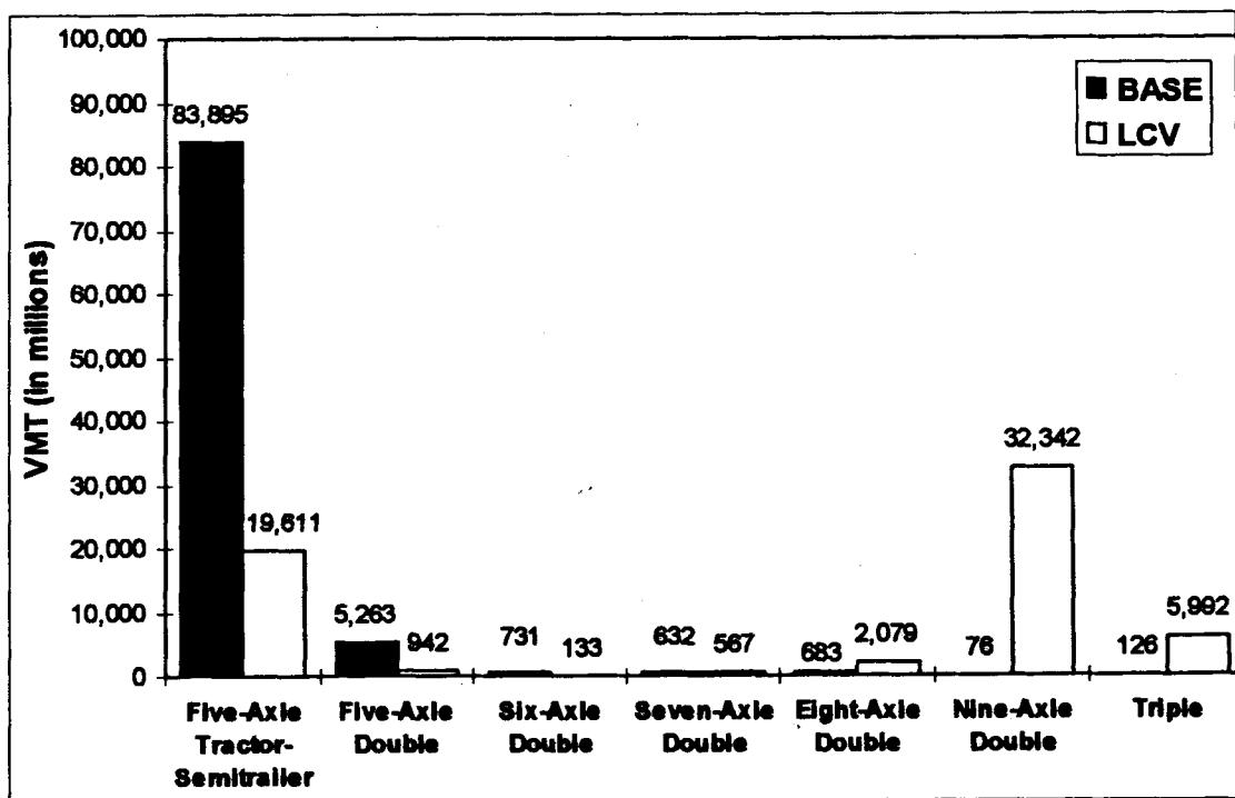
EXHIBIT 4-17 COMPARISON OF VEHICLE-MILES-OF-TRAVEL (YEAR 2000) BASE CASE AND LONGER COMBINATION VEHICLES NATIONWIDE SCENARIO
