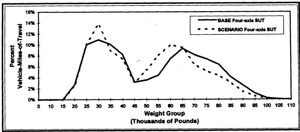
EXHIBIT 4-5 WEIGHT DISTRIBUTION EXAMPLE BASE CASE AND UNIFORMITY SCENARIO FOUR-AXLE SINGLE UNIT TRUCK
